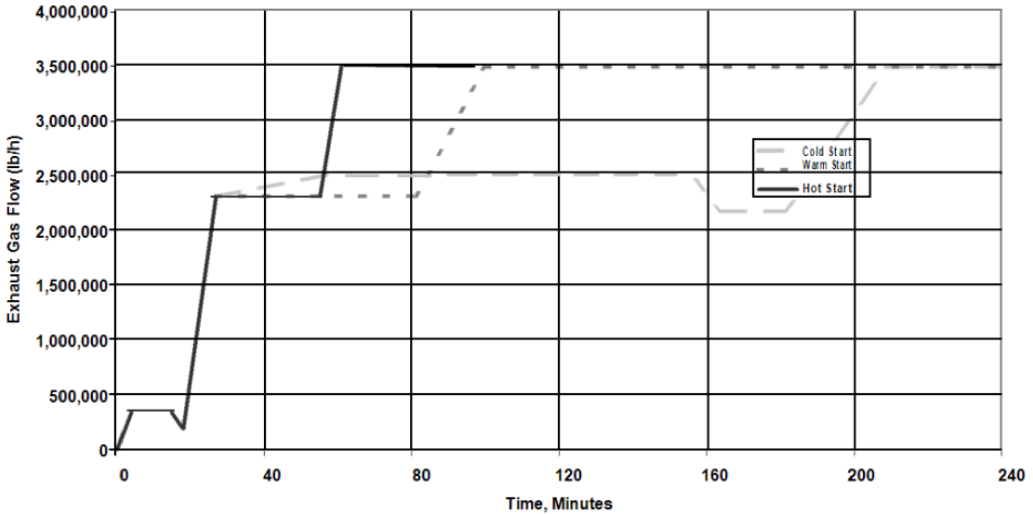
Figure 1b - Typical Frame 7 Gas Turbine Exhaust Flows
