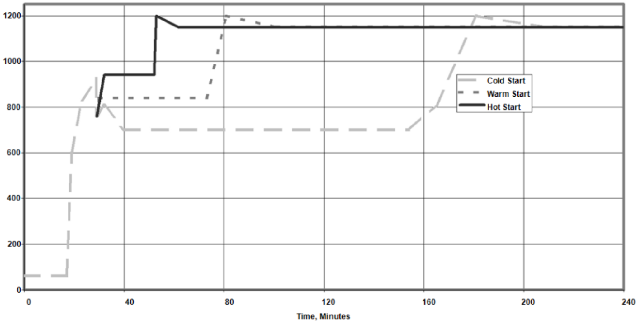
Figure 1a - Typical Frame 7 Gas Turbine Exhaust Temperatures
